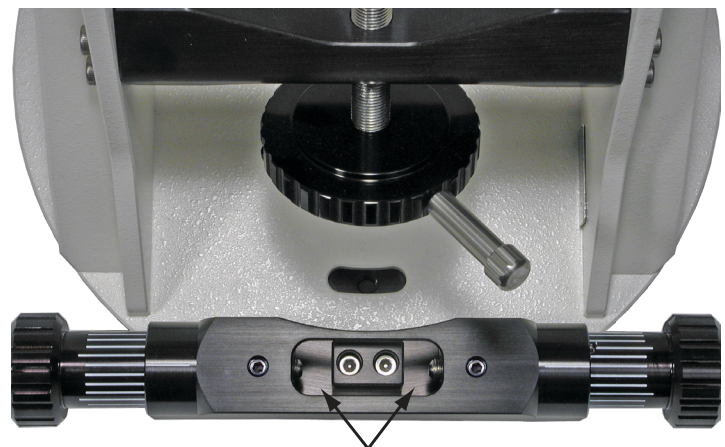
Allow Space for Azimuth Adjuster Block
