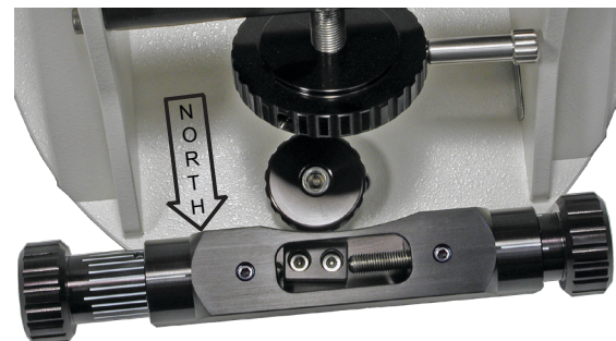
Pier East of True North - Adjusted West
