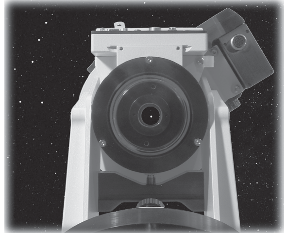
Sighting Polaris through Polar Alignment Sight Hole
