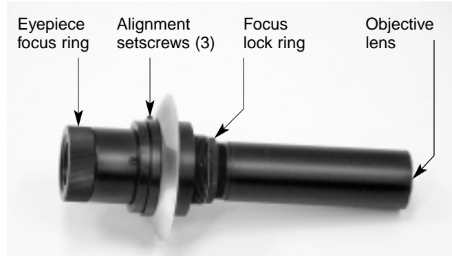
Figure 9. The optional polar axis finder scope.
