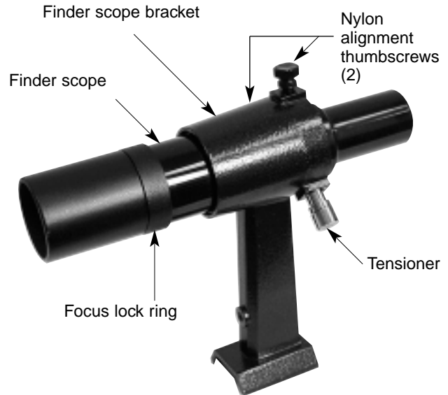
Figure 3a. The 6x30 finder scope.
