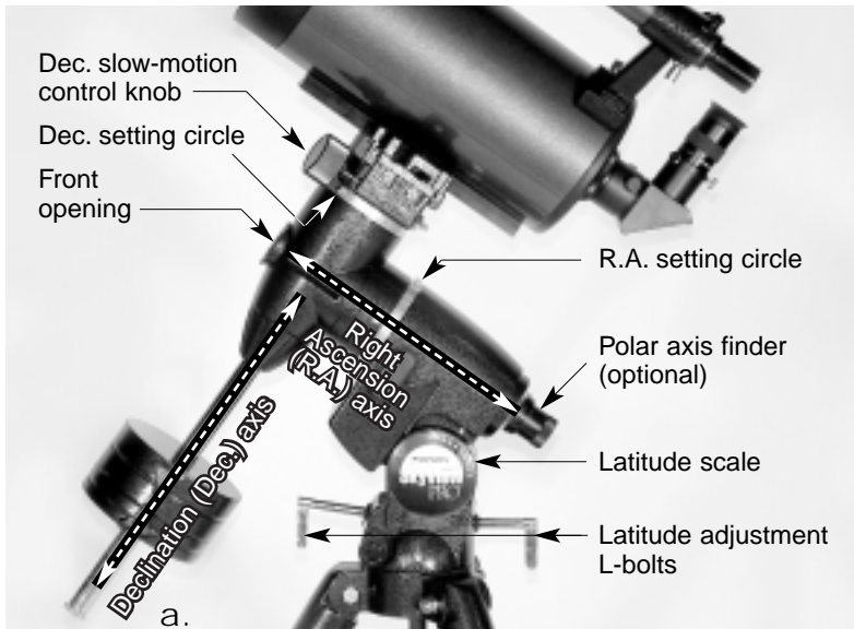
Figure 6a-b. The SkyView Pro 127mm EQ mount.
