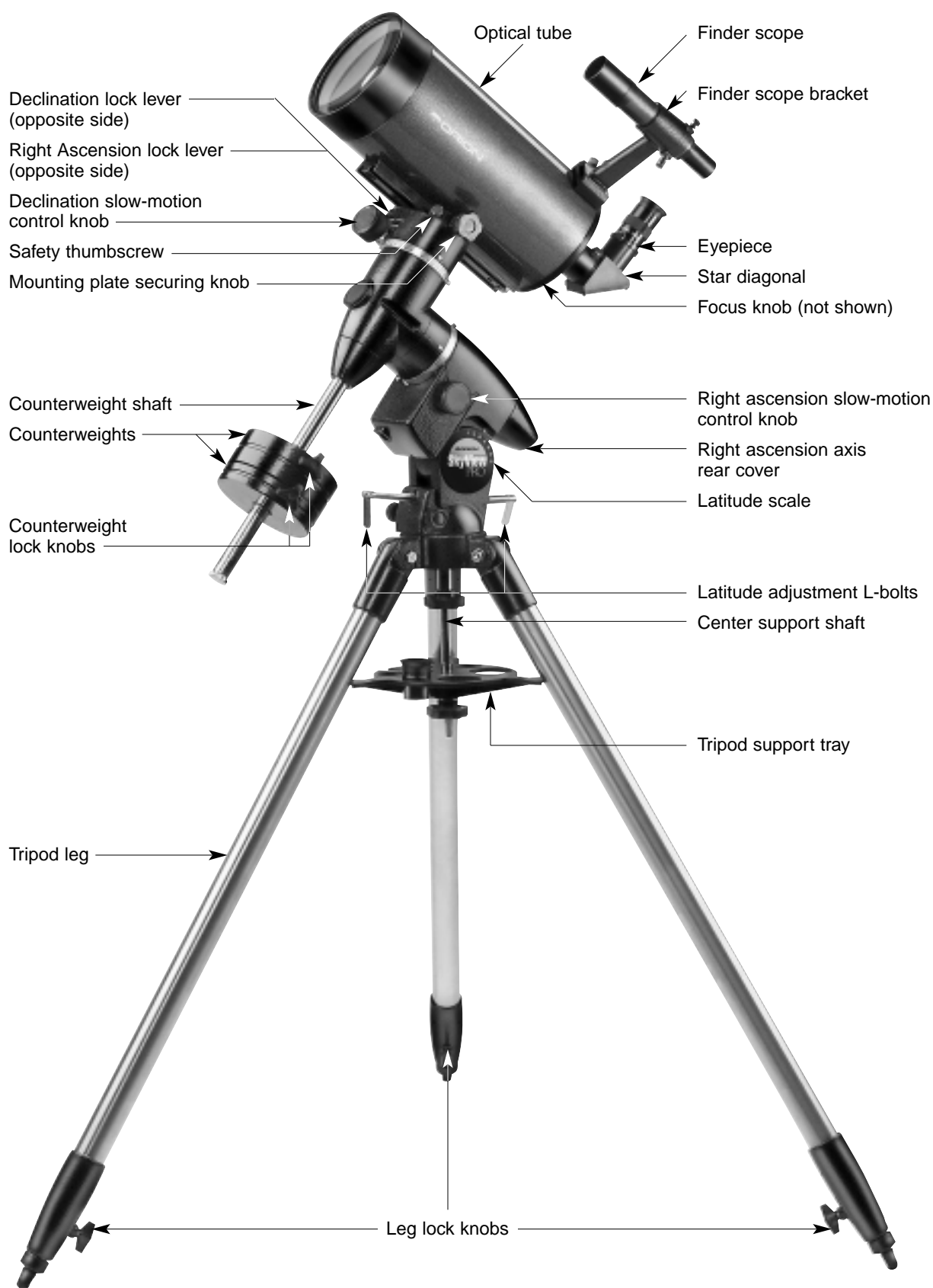
Figure 1. The SkyView Pro 127mm EQ.
