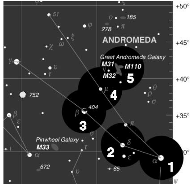
Figure 21. Starhopping is a good way to locate hard-to-find objects. Refer to a star chart to map a route to the object that uses bright stars as guideposts. Center the first star you've chosen in the finder scope and telescope eyepiece (1). Now move the scope carefully in the direction of the next bright star (2), until it is centered. Repeat (3 and 4). The last hop (5) should place the desired object in the eyepiece.
