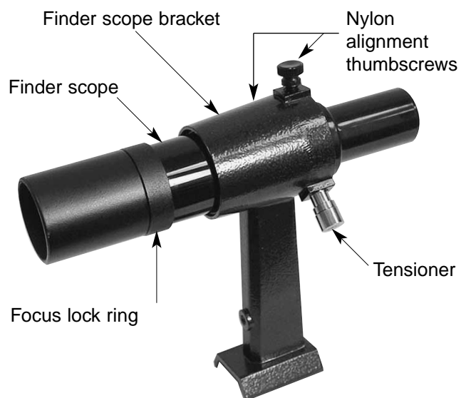
Figure 3a. The 6x30 finder scope.
