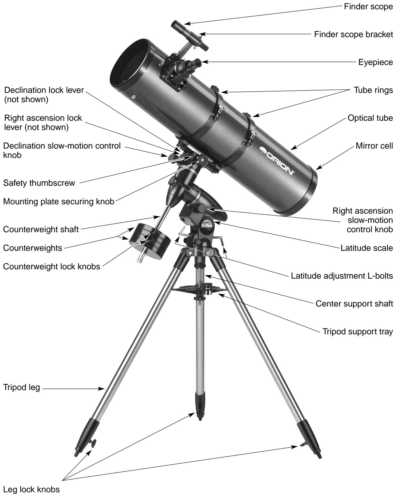
Figure 1. The SkyView Pro 8 EQ.
