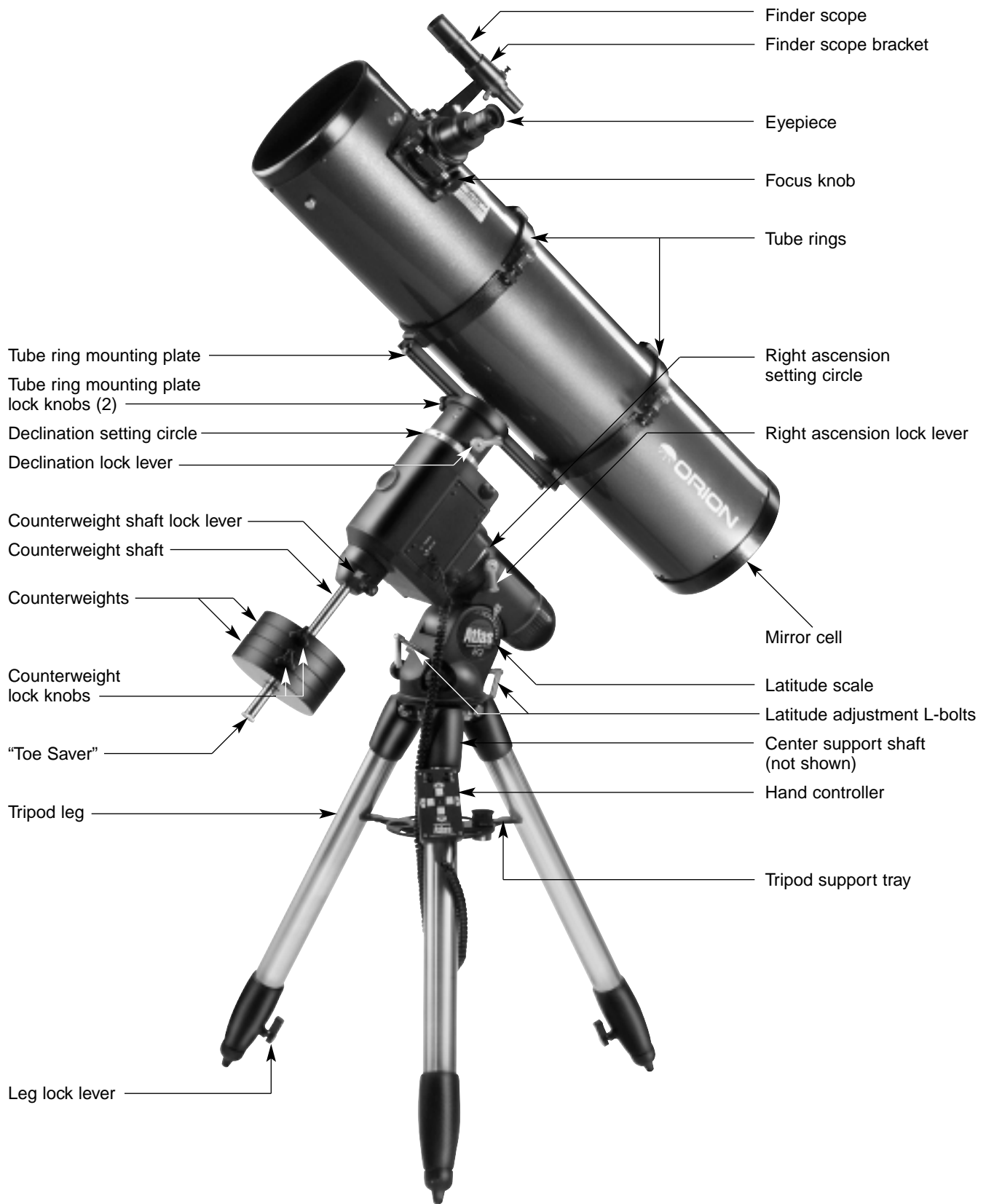
Figure 1. The Atlas 8 EQ.
