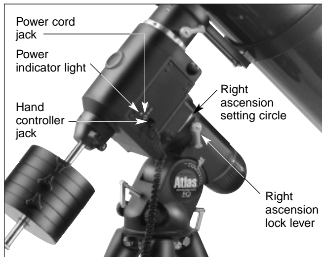
Figure 1b. The Atlas 8 EQ mount.
