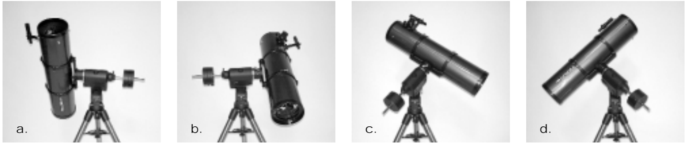
Figure 13a-d. These illustrations show the telescope pointed in the four cardinal directions. (a) north, (b) south, (c) east, (d) west. Note that the tripod and mount have not been moved; only the telescope has been moved on its R.A. and Dec. axes.
