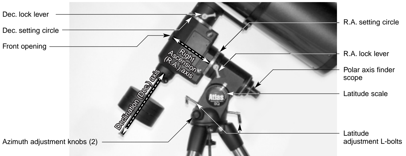
Figure 7. The Atlas EQ Mount.
