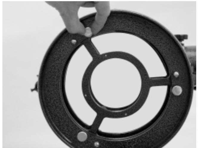
Figure 18. The tilt of the primary mirror is adjusted by turning one or more of the three larger thumbscrews.
