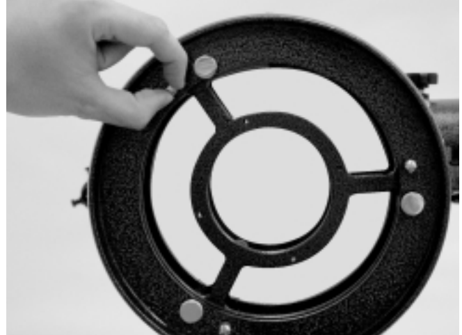
Figure 17. The three small thumbscrews that lock the primary mirror in place must first be loosened before any adjustments can be made.
