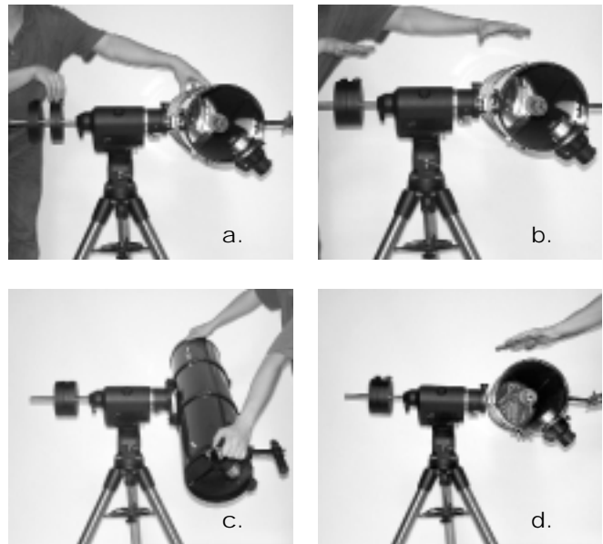
Figure 5a-d. Proper operation of the equatorial mount requires that the telescope tube be balanced on the R.A. and Dec. axes. (a) With the R.A. lock lever released, slide the counterweights down the counterweight shaft until they just counterbalance the telescope tube. (b) When you let go with both hands, the tube should not drift up or down. (c) With the Dec. lock lever released, loosen the tube ring lock clamps a few turns and slide the telescope forward or back in the tube rings. (d) When the tube is balanced about the Dec. axis, it will not move when you let go.
