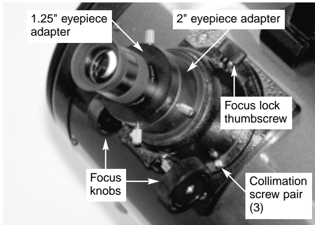
Figure 4. The 2" focuser of the Atlas 8 EQ.
